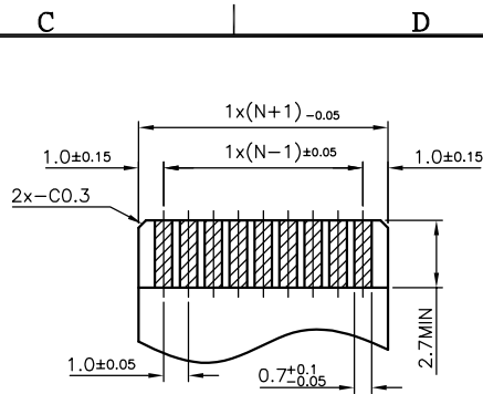
APPLICABLE RECOMMENDED LAYOUT (THICKNESS:0.3±0.05)
